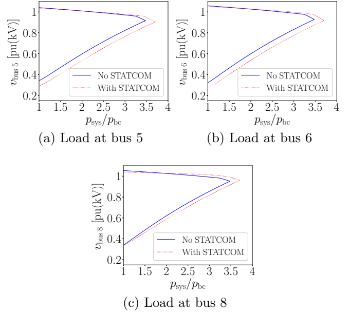
Fig. 5. pv curves at the load buses of the modified WSCC 9-bus system with and without a STATCOM. The x-axis represents the ratio between the loading level of the system, p_{sys} , and the base-case condition, p_{bc} .
