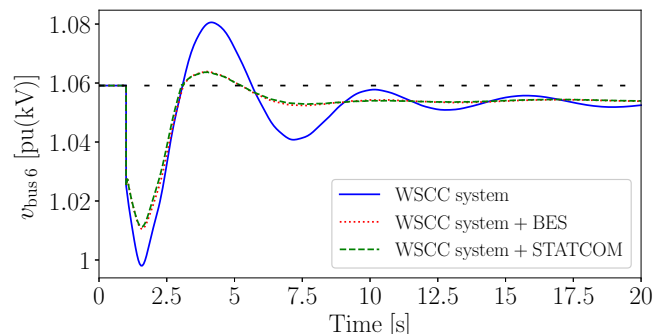
(b) Voltage at the load bus 6
