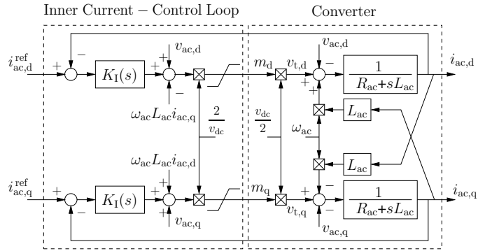
Fig. 2. Block diagram of the VSC inner current-control and converter in the dq frame.
