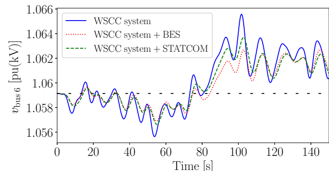
(b) Voltage at the load bus 6
