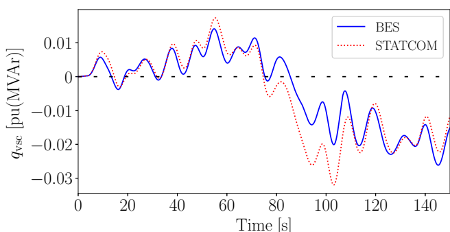
(c) Reactive power output of the VSC
