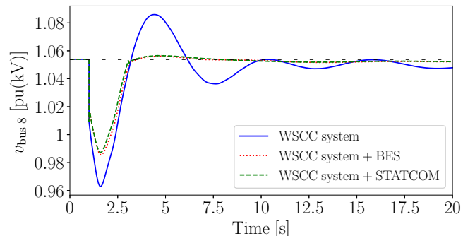
(a) Voltage at the PCC
