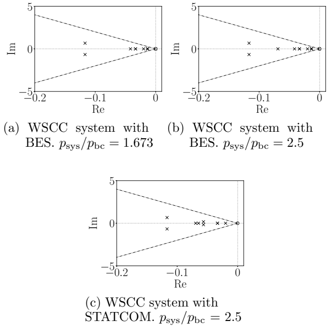
Fig. 8. Eigenvalue loci of the rightmost eigenvalues of the WSCC system with a BES and a STATCOM. Dash-dot lines indicate 5% damping.
