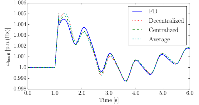
Fig. 7. Frequency of bus 6 after a three-phase fault. No communication delays are considered.
